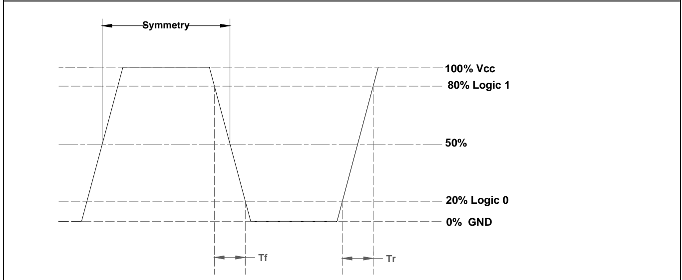
WAVEFORM: LOAD = 15pF
