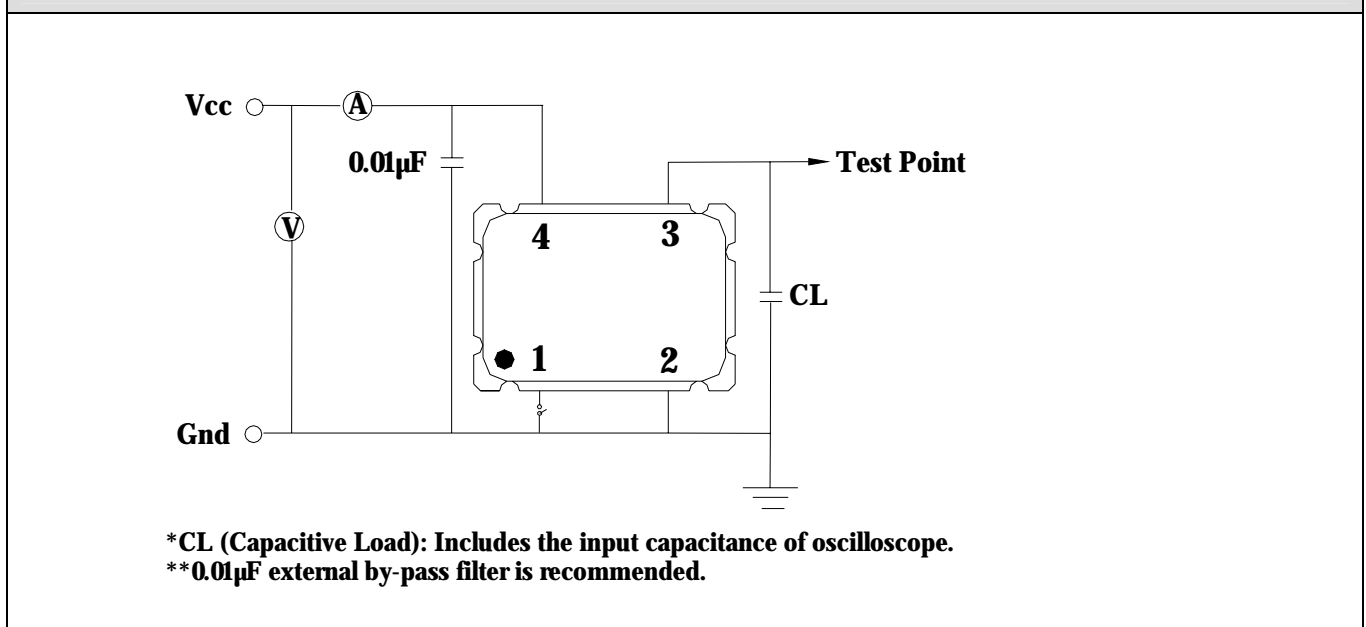
RECOMMENDED TEST CIRCUIT WITH CMOS LOAD:
